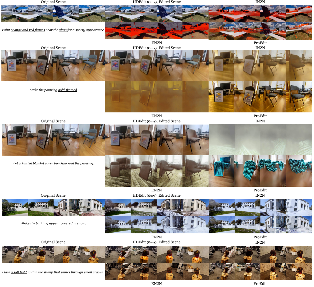
Figure I. Our HDEdit achieves high-quality editing results across various indoor and outdoor scenes, consistently fulfilling editing instructions while preserving original content for all the tasks. In contrast, the baselines either fail to complete the editing or alter many unrelated regions without adequate preservation. Please refer to Project Page for the rendered videos.
