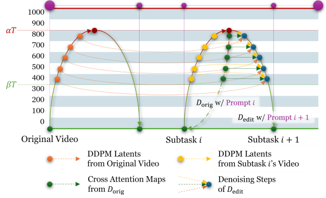
Figure G. When moving forward to the next subtask, our HDEdit performs a parallel denoising control. By reusing the information from previous denoising steps, we effectively preserve the necessary information.
